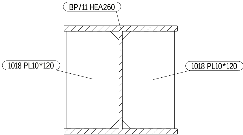
A - A 1:5
